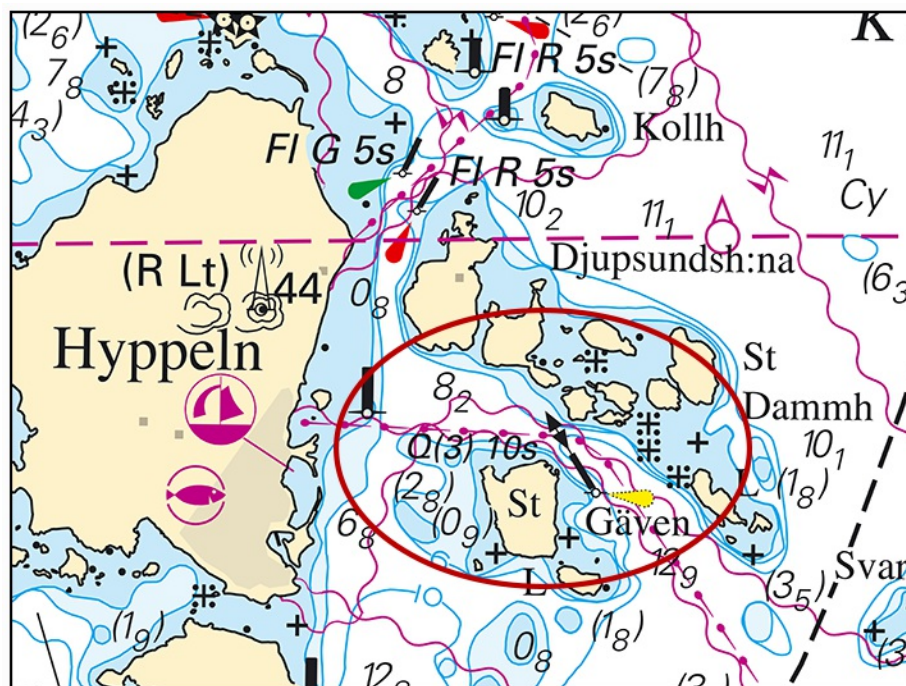
Amended buoyage at Hyppeln in Göteborgs northern archipelago
